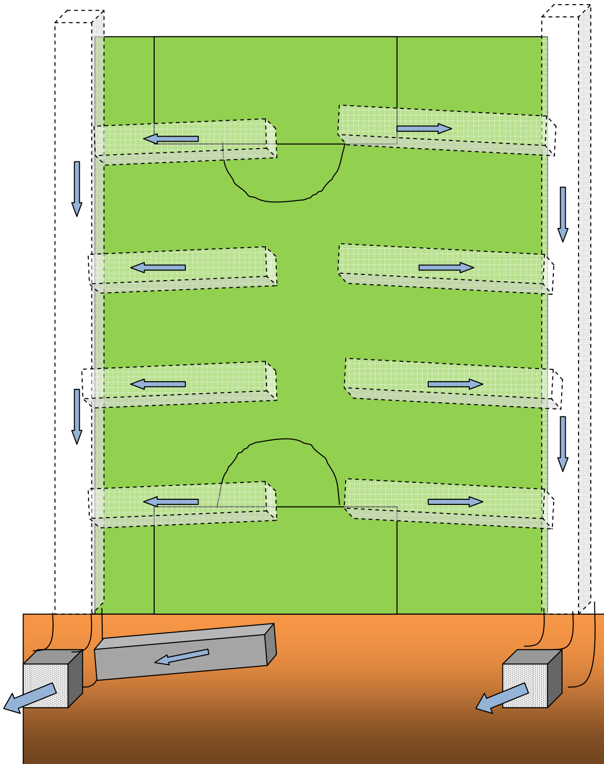
SOCCER FIELD DRAINAGE SYSTEM USING IDROSAC 500
